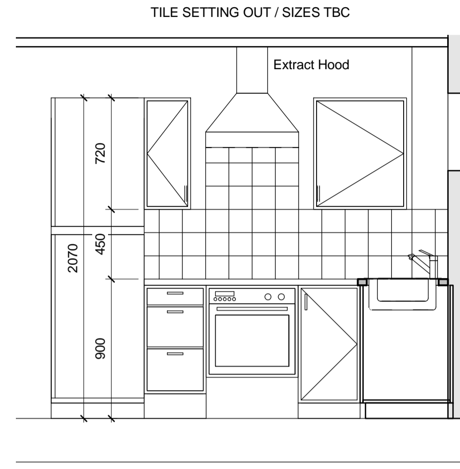
H1 Elevation H1 1 : 25
