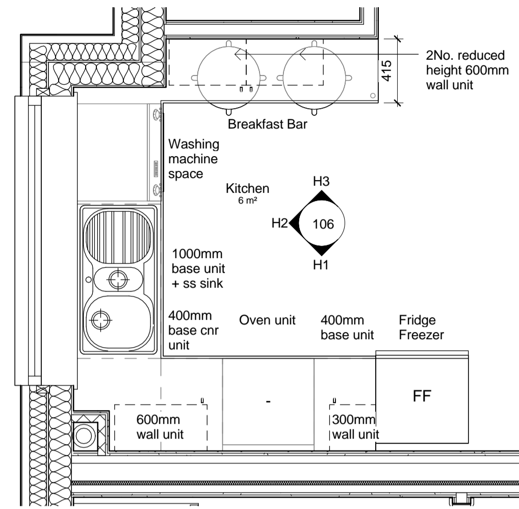
2 Flat Type H Kitchen 1 : 25
