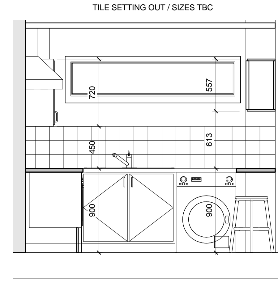
H2 Elevation H2 1 : 25
