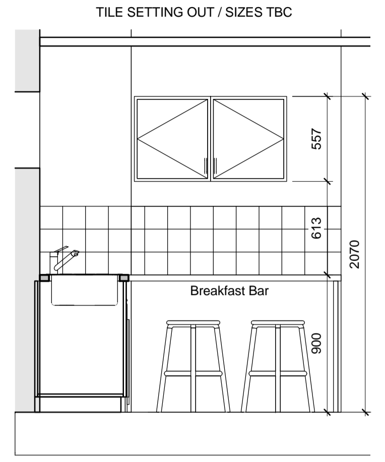
H3 Elevation H3 1 : 25
