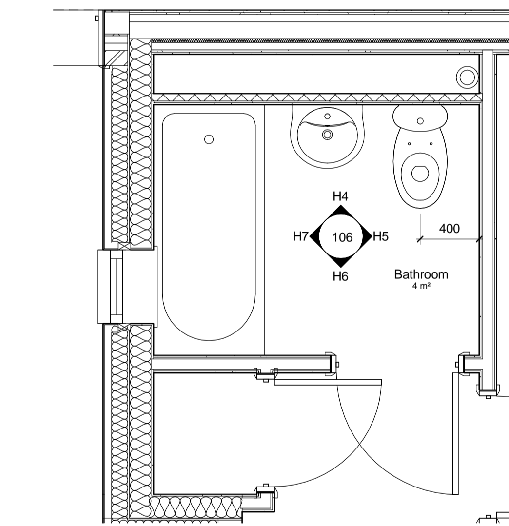
3 Flat Type H Bathroom 1 : 25
