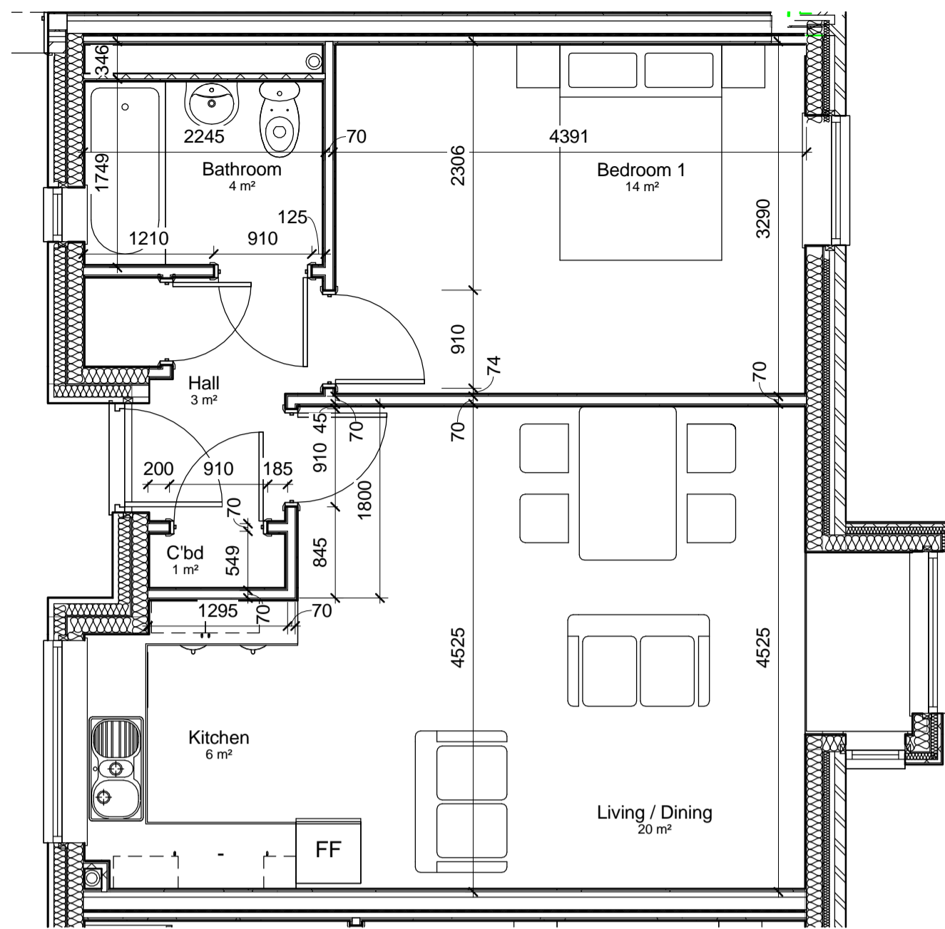
1 Flat Type H 1 : 50 FLATS 8, 16 & 24 Note: All dimensions taken to stud face
