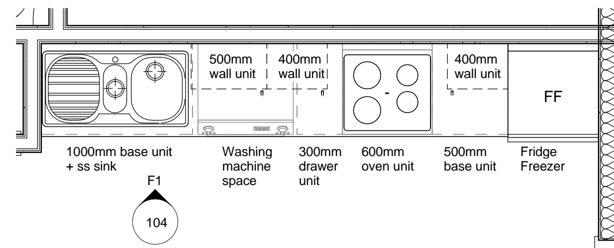
2 Flat Type F Kitchen 1 : 25
