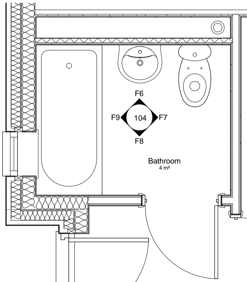
3 Flat Type F Bathroom 1 : 25
