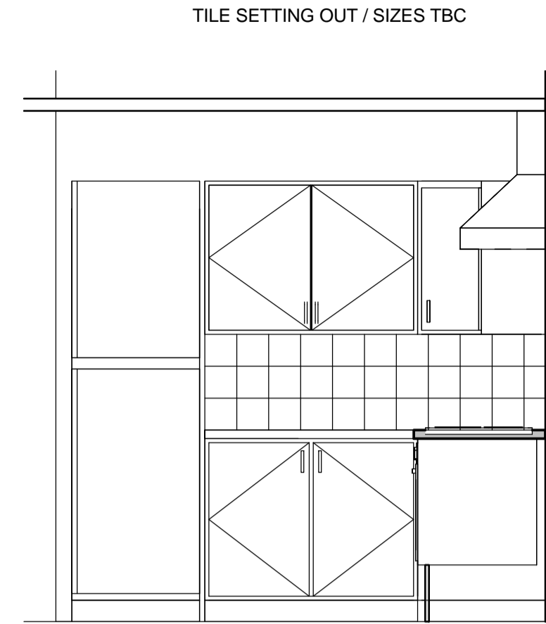
B1 Elevation B1 1 : 25
