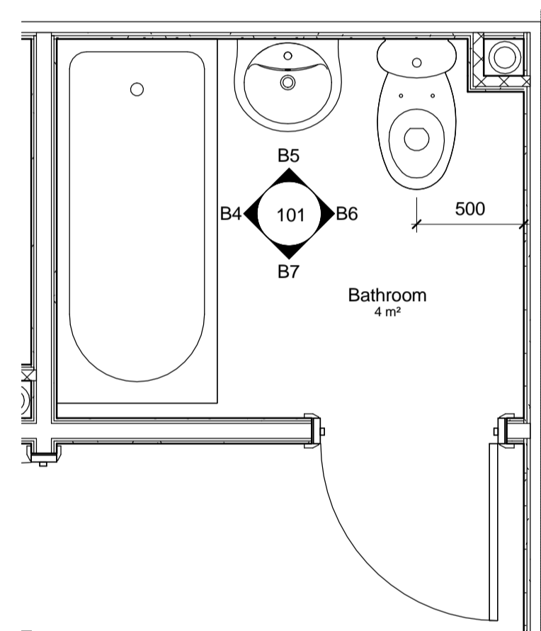
3 Flat Type B Bathroom 1 : 25
