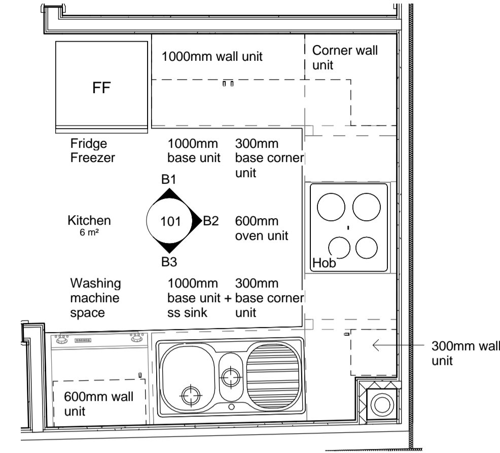
2 Flat Type B Kitchen 1 : 25
