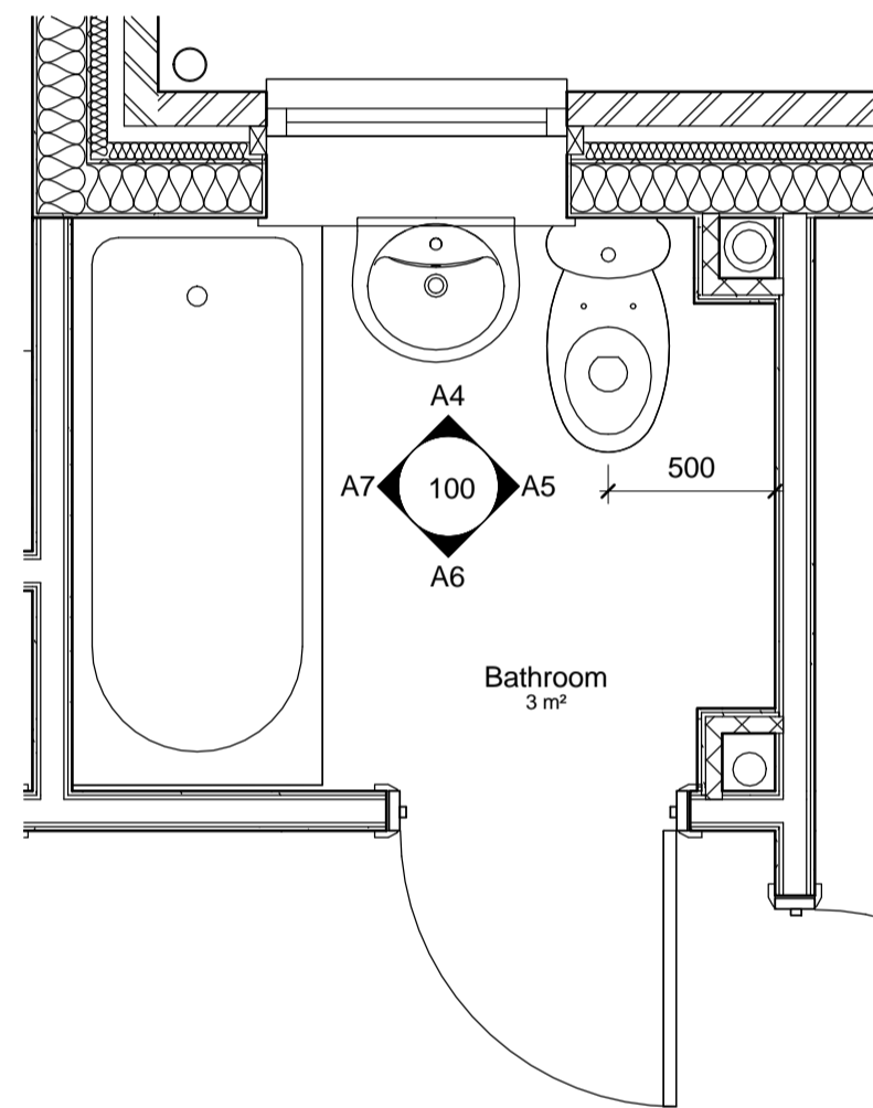
3 Flat Type A Bathroom 1 : 25
