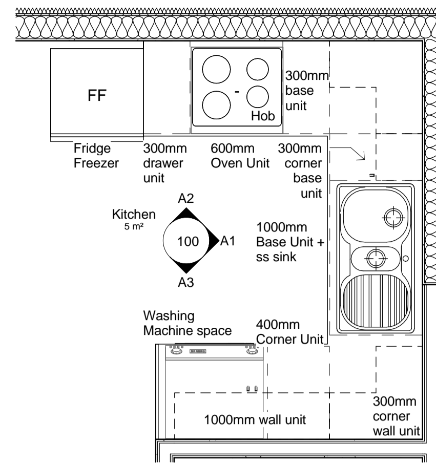
2 Flat Type A Kitchen 1 : 25
