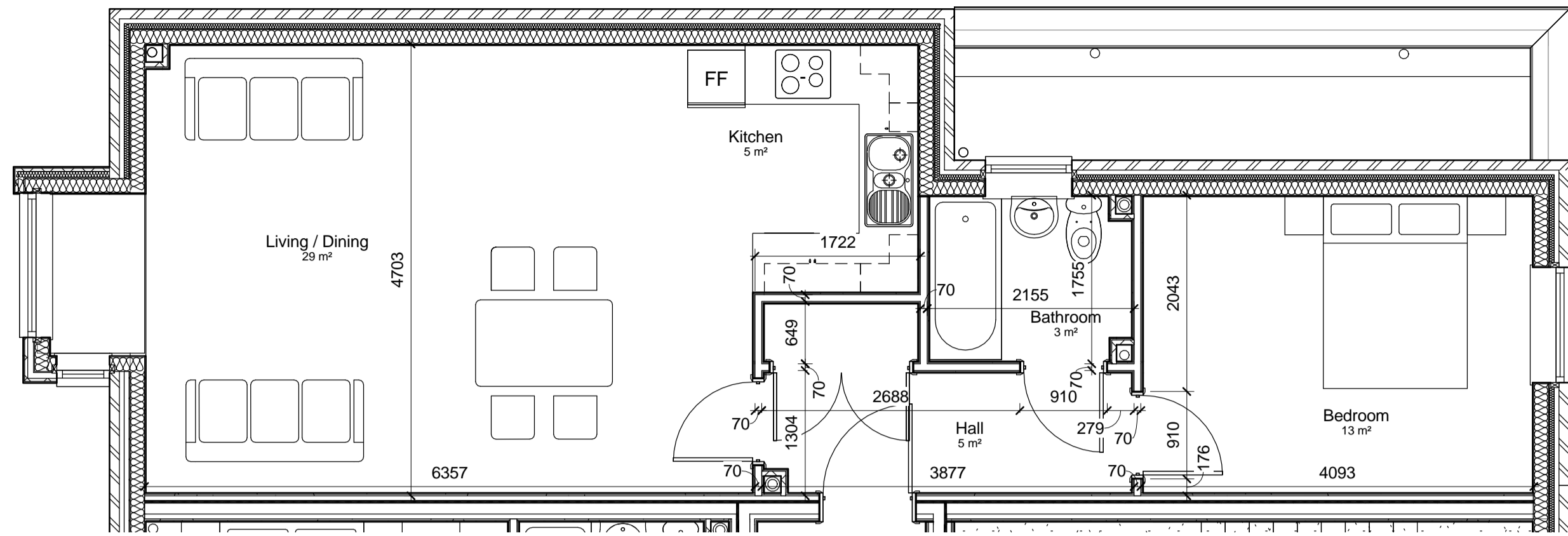
1 Flat Type A 1 : 50 FLATS 1, 9 & 17 Note: All dimensions taken to stud face
